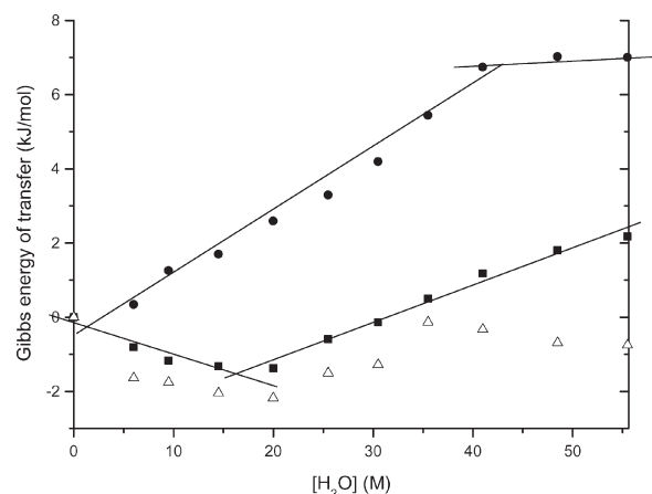
Figure 6. Gibbs energies of transfer ( \Delta_{tr}G^\circ ) for 1 (●), MVK (■) and the AC (△), for the reaction of 1 with MVK in mixtures of water with 1-propanol (relative to 1-propanol) 4
