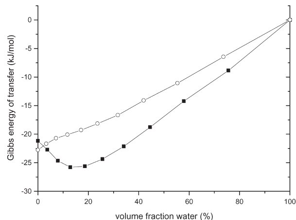
Figure 7. Gibbs energies of transfer ( \Delta_{tr}G^\circ ) for betaine-30 from water to mixtures of water with acetonitrile (■) or ethanol (○), calculated from solubility data 39
